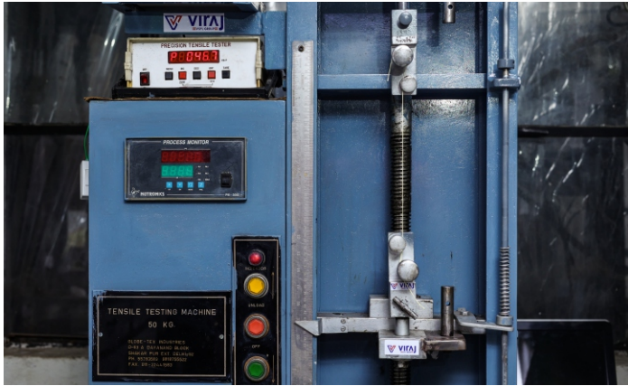
Digital Yarn Tensile Testing , Capacity 50 kgf
