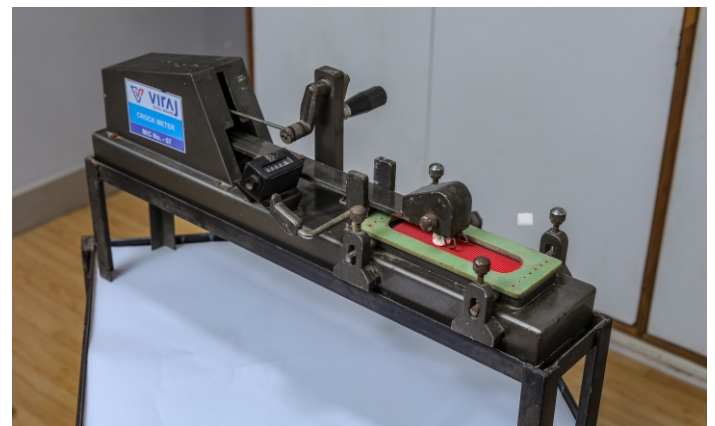
Crock Meter/Rubbing-Wet & Dry
